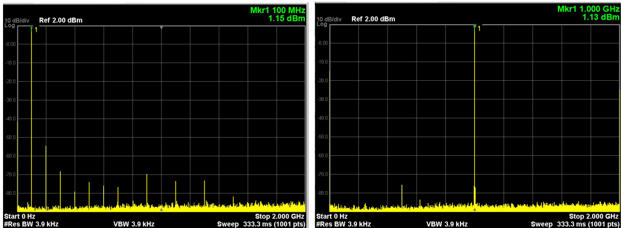
Figure 1. (Left) Measured IQ output, 100 MHz tone spectrum. (Right) Measured IQ output, 1 GHz tone spectrum.
