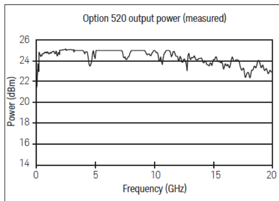
Maximum available power in CW mode (measured)
