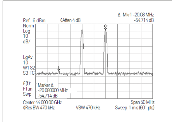
44 GHz two-tone (measured)
