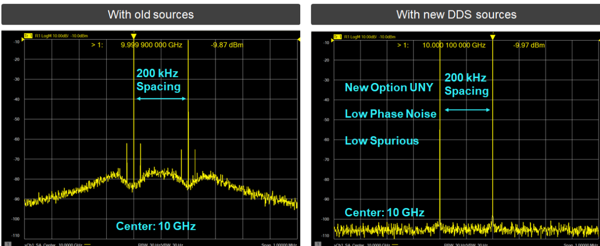
Figure 6. Two-tone measurements
