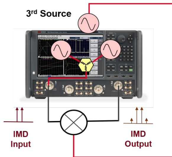
Figure 7. Two-tone IMD mixer measurement
