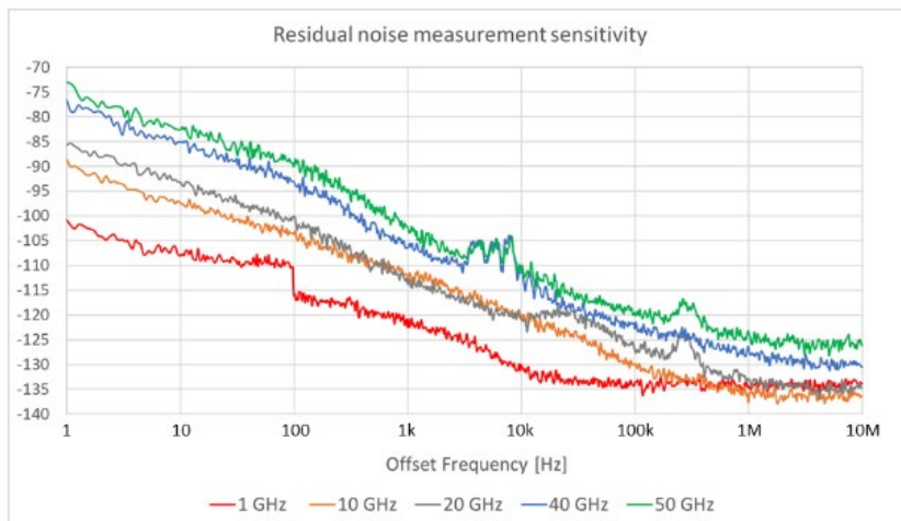
Figure 15. PNA residual noise measurement noise floor
