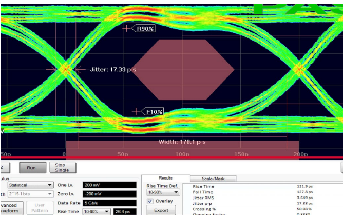
Figure 30. The simulated eye diagram analysis capability eliminates the need for a pulse pattern generator.
