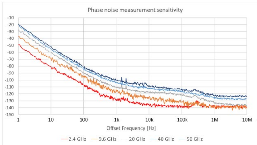
Figure 14. PNA Phase noise measurement noise floor
