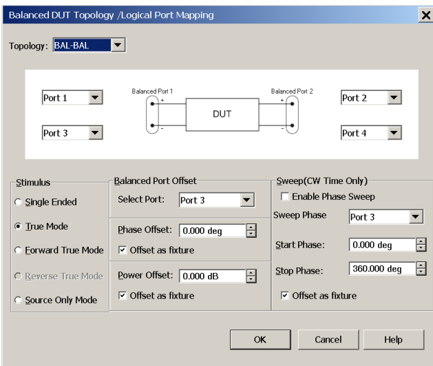
Figure 27. Various stimulus and sweep settings are available in the Balanced DUT Topology dialog, allowing you to select the right configuration for all of your balanced devices.
