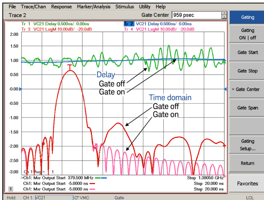
Figure 9. Time-domain gating can remove ripple by removing unwanted, time-delayed responses due to spurious signals.
