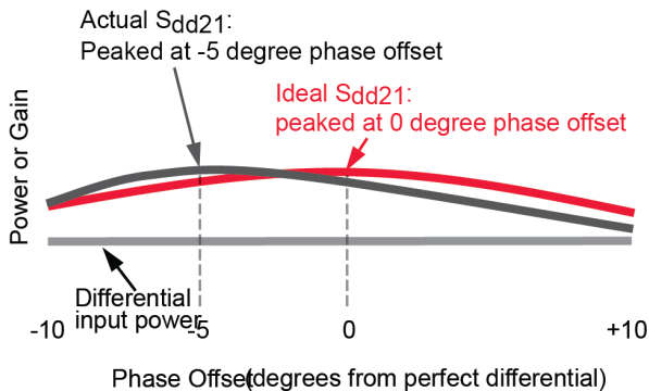
Figure 28. In-fixture phase-offset sweeps reveal the optimal phase offset to achieve the highest amplifier gain, which is essential to the design of the input matching circuit.
