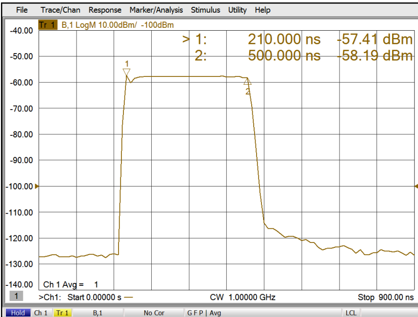
Figure 5. Pulse profile measurement using narrowband detection technique allows 30 measurement points within 300 ns pulse, with 10 ns timing resolution.
