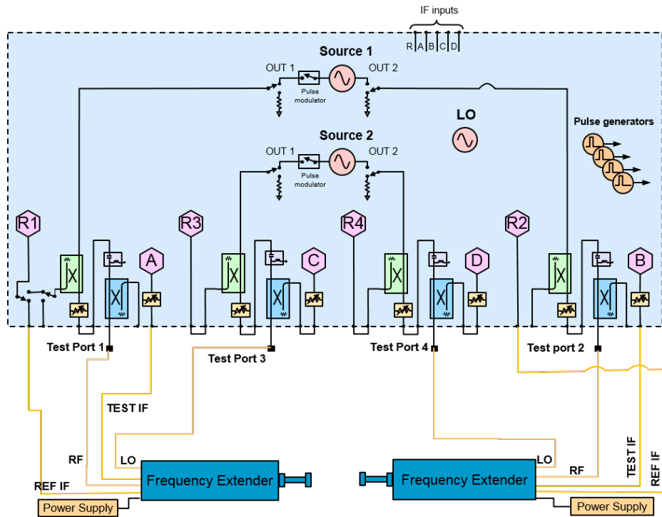
Figure 34. Block diagram of a two-port millimeter-wave system using a four-port PNA and two millimeter-wave frequency extenders.
