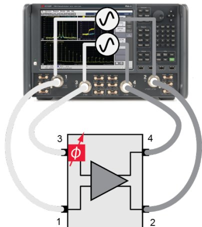
Figure 24. Without mismatch correction, the delivered signals to the DUT will not be truly differential due to reflection from the DUT input and the subsequent re-reflection from the sources. This effect can be corrected with mismatch correction.
