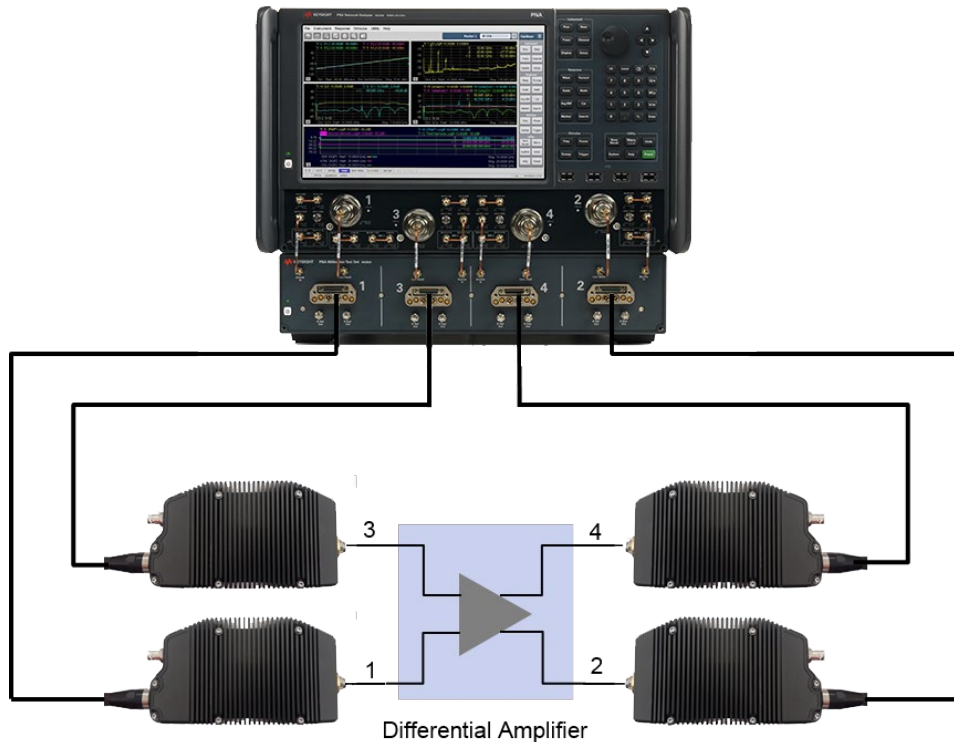
Figure 37. True-differential measurement of a balanced trans-impedance amplifier using a four-port PNA, the N5292A controller, and N5293A frequency extenders.
