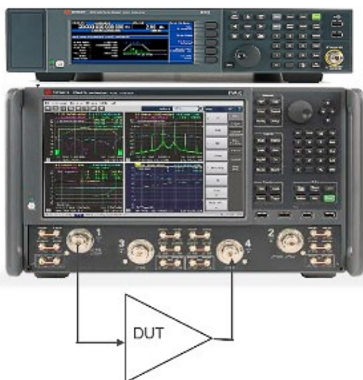
Classic NPR measurement with PNA-X and UXG
