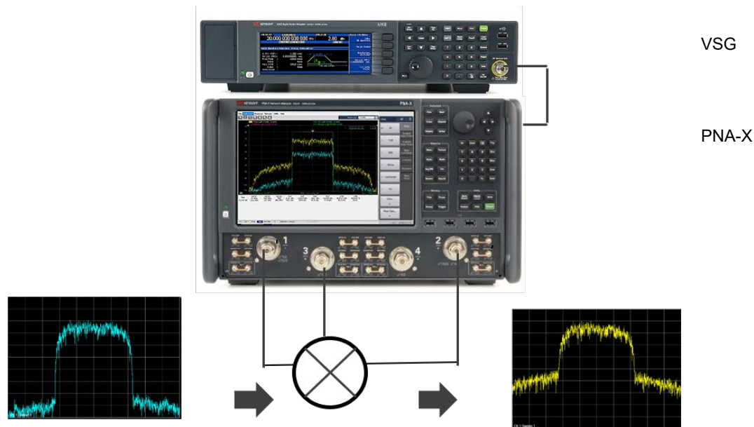
Figure 21. Mixer EVM/NPR/ACPR measurement with Modulation distortion application
