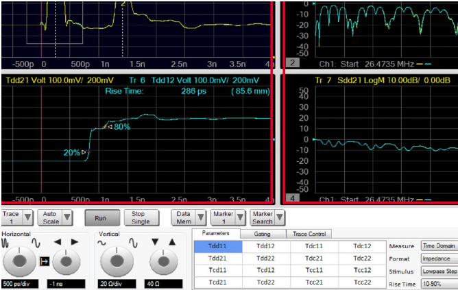
Figure 29. Measurements are taken as a function of frequency. The frequency domain information is used to calculate the Inverse Fourier Transform for time domain results.
