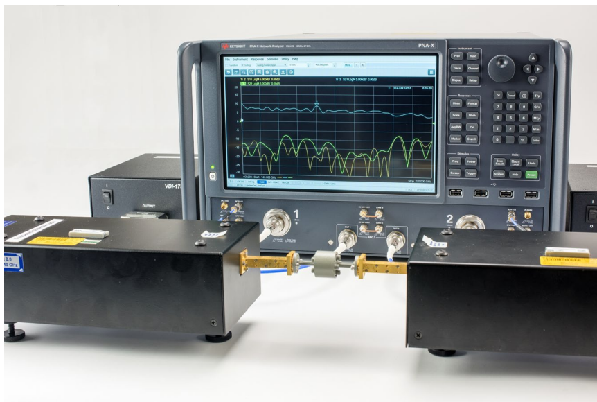
Figure 33. Direct connection of VDI modules to a four-port PNA-X enables S-parameter measurements to 1.5 THz.
