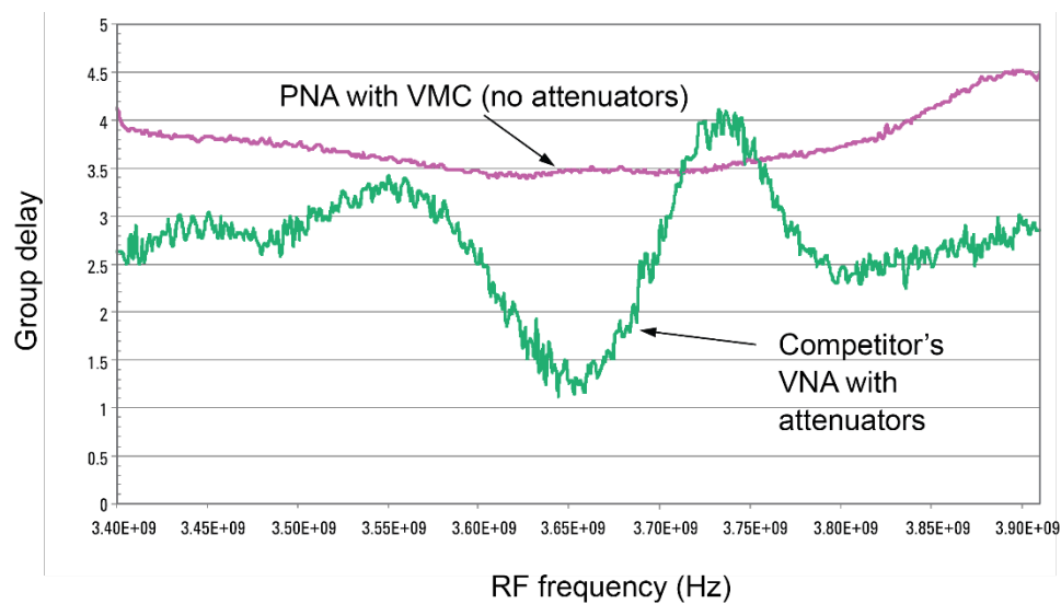
Figure 11. VMC's match correction greatly reduces mismatch errors in group delay measurements, eliminating the need for attenuators at the ends of the test cables.
