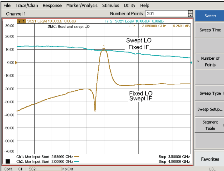
Figure 8. With two internal signal sources, the PNA-X provides fast measurements of both fixed and swept IF responses.
