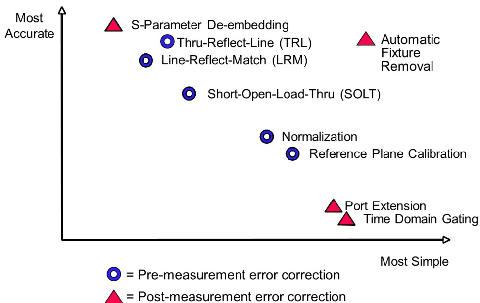
Figure 31. A relative comparison of various fixture error-correction methods
