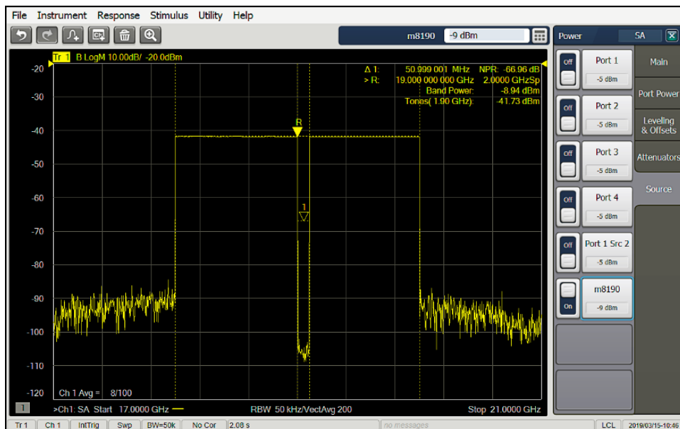
Figure 17. Improved flatness and lower noise floor in the notch after signal correction
