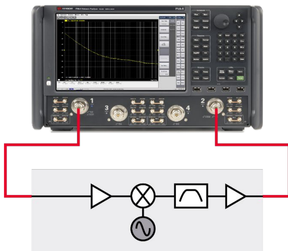
Embedded-LO frequency converter
