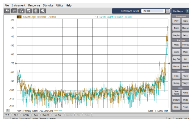
Figure 35. 100 dB dynamic range 750 GHz to 1.1 THz (IFBW = 10 Hz)
