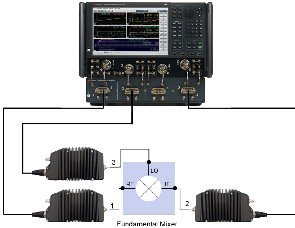
Figure 36. A dual-source PNA with an N5292A four-port controller and broadband frequency-extender modules characterize mixers and converters at millimeter wave frequencies. The PNA's second source can be used to provide an LO signal to a mixer.
