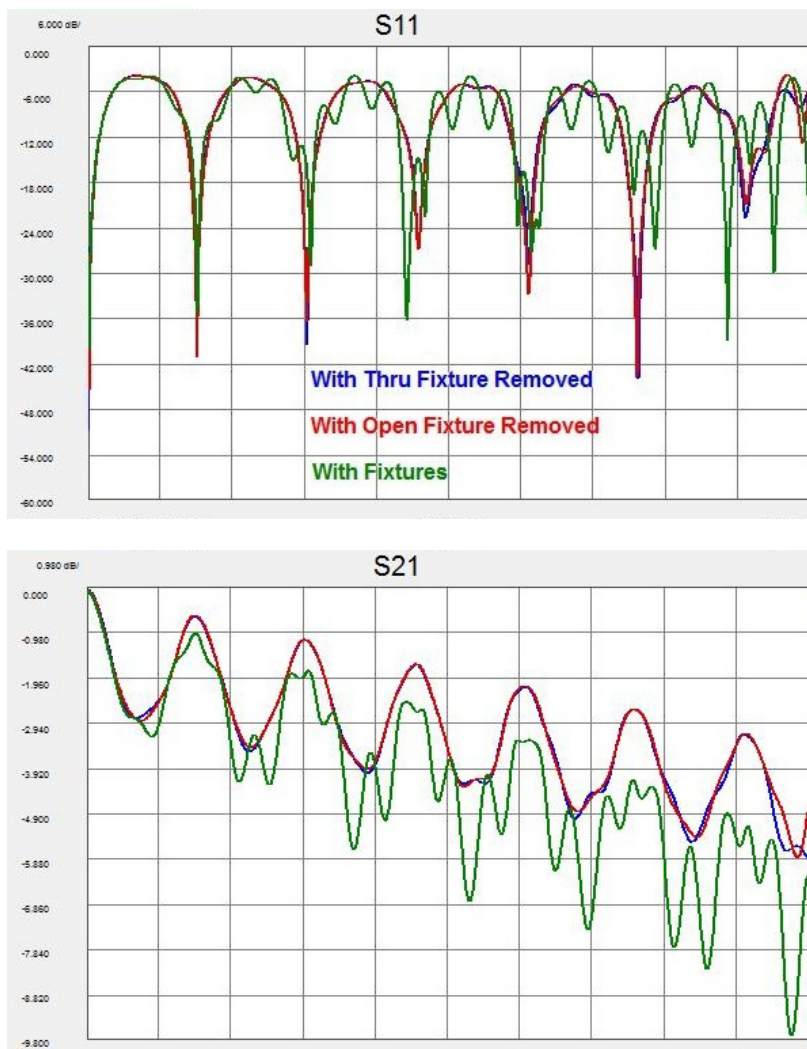
Figure 32. S11 and S21 in frequency domain
