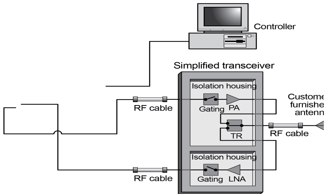
Figure 39. PNA-X configured for radar cross-section measurements
