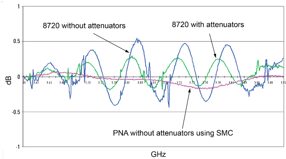
Figure 10. SMC's match correction greatly reduces mismatch errors in conversion loss/gain measurements, eliminating the need for attenuators at the ends of the test cables.
