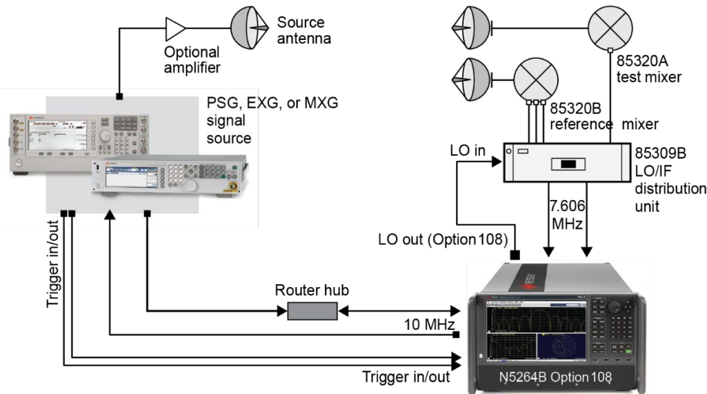
Figure 41. PNA-X measurement receiver configured for far-field measurements (PNA-X Option 020 with IF inputs can also be used).
