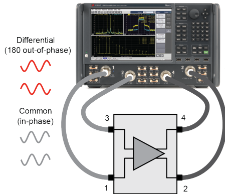
Figure 22. Using the PNA-X's two internal sources, iTMSA drives the differential amplifier under real world conditions, providing accurate mixed-mode S-parameters in all operating environments.
