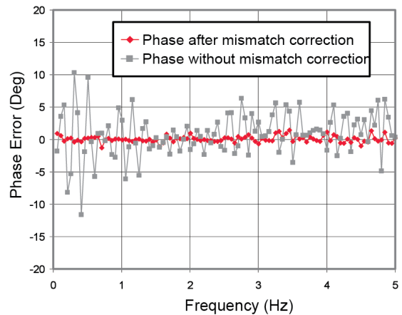
Figure 25. iTMSA compensates for mismatch errors by measuring the raw matches of the VNA and DUT, and precisely adjusting the amplitude and phase of the two signals at the reference plane to achieve ideal true-mode signals.
