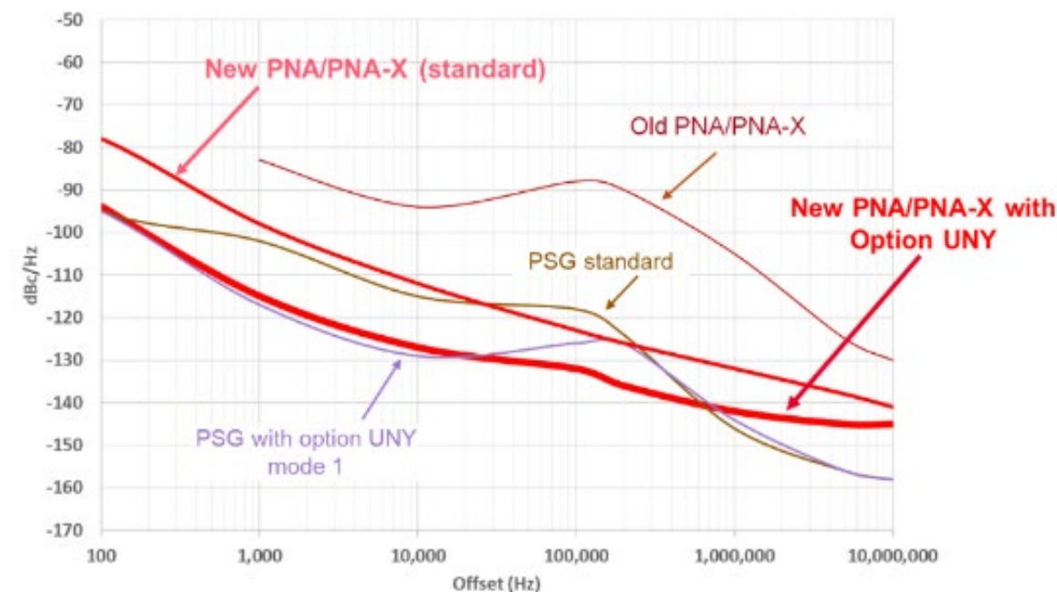
10 GHz phase noise comparison
