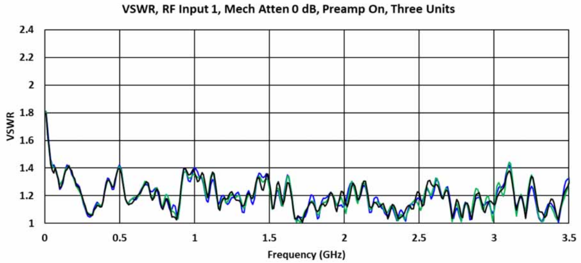
Nominal VSWR - Input 1 - Preamp On Band [Plot]
