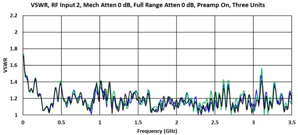
Nominal VSWR - Input 2 - Preamp On Band [Plot]
