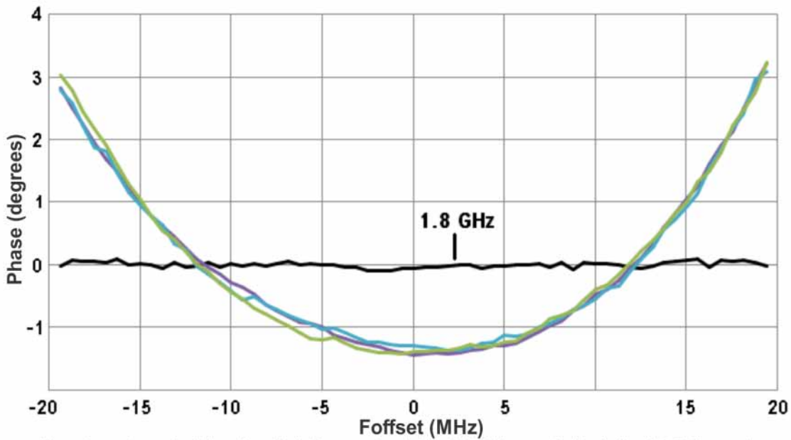
Nominal Phase Linearity [Plot]
